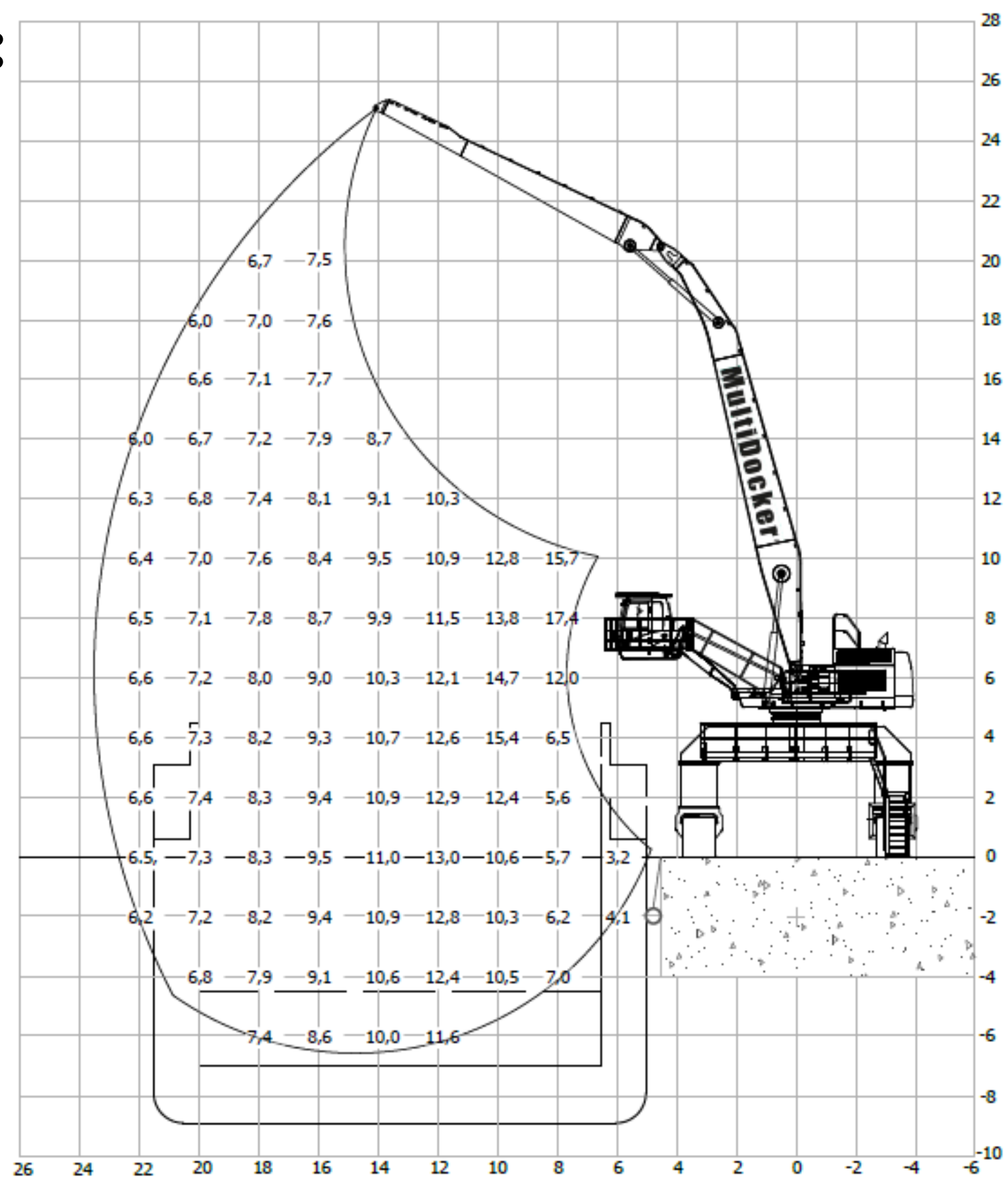
Lifting capacity table, unit tonne = 1.000 kg The lifting capacities are measured at 360° in the stick end-joint. The above values have been calculated in compliance with SS-EN 13001. They do not exceed 87% of the hydraulic lifting capacity or 75% of the tipping load, with the machine on firm, level ground.
